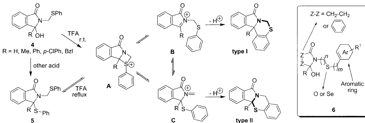
Scheme 2. The mechanism of the tandem intramolecular sulfuration/isomerization/ \pi -cationic cyclization process.
