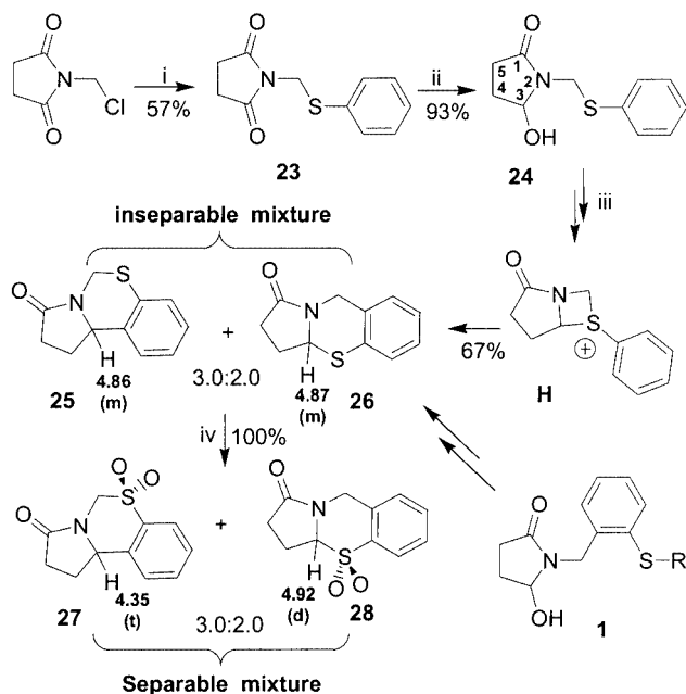
Scheme 8. Effect of the nature of the N -acyliminium species: (i) 1.0 equiv. of thiophenol, NaH, DMF, 5 h; (ii) 6 equiv. of \text{NaBH}_4 , MeOH, 0 °C, 35 min; (iii) neat TFA, room temp., 2 h; (iv) 2.2 equiv. of m -CPBA, \text{CH}_2\text{Cl}_2 , 0 °C to room temp., 2 min and 1 h.
