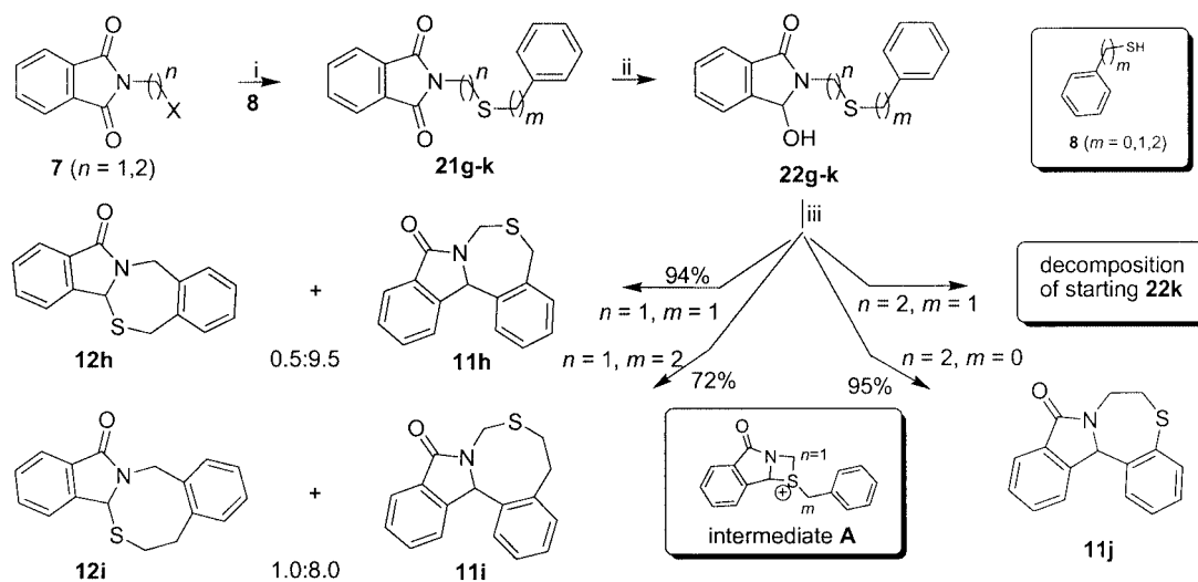
Scheme 5. Conditions and reagents: (i) MeONa, DMF, 1.5 equiv. of thiol derivative 8 , room temp., 5 h; (ii) 4 to 6 equiv. of NaBH 4 , MeOH, 0 °C, 30 to 45 min; (iii) neat TFA, 24 h.
