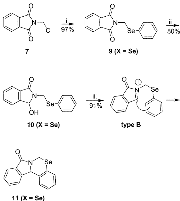
Scheme 7. Influence of the heteroatom on the cyclization: (i) 1.1 equiv. of selenophenol, MeONa, DMF, 12 h; (ii) 5 equiv. of \text{NaBH}_4 , MeOH, 0 °C, 45 min; (iii) neat TFA, room temp., 3 h.
