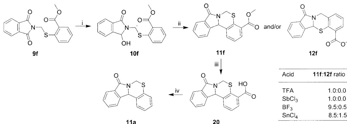
Scheme 4. Conditions and reagents: (i) 4 equiv. of NaBH 4 , MeOH, 0 °C, 35 min; (ii) See conditions in table; (iii) K 2 CO 3 , MeOH/H 2 O, 5:1, reflux, 3 h; (iv) Cu, quinoline, 150 °C, 3.5 h.
