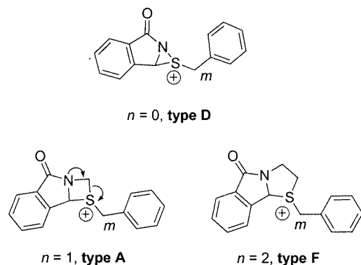
Scheme 6. Azasulfonium ions as potential intermediates in the tandem cyclization process.
