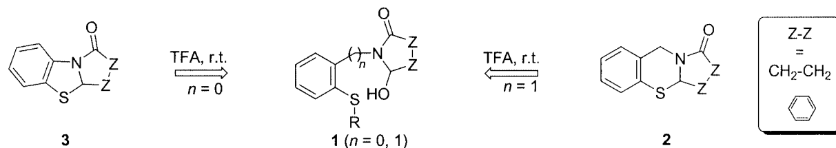
Scheme 1. Heterocyclization with the sulfur atom as internal nucleophile.
